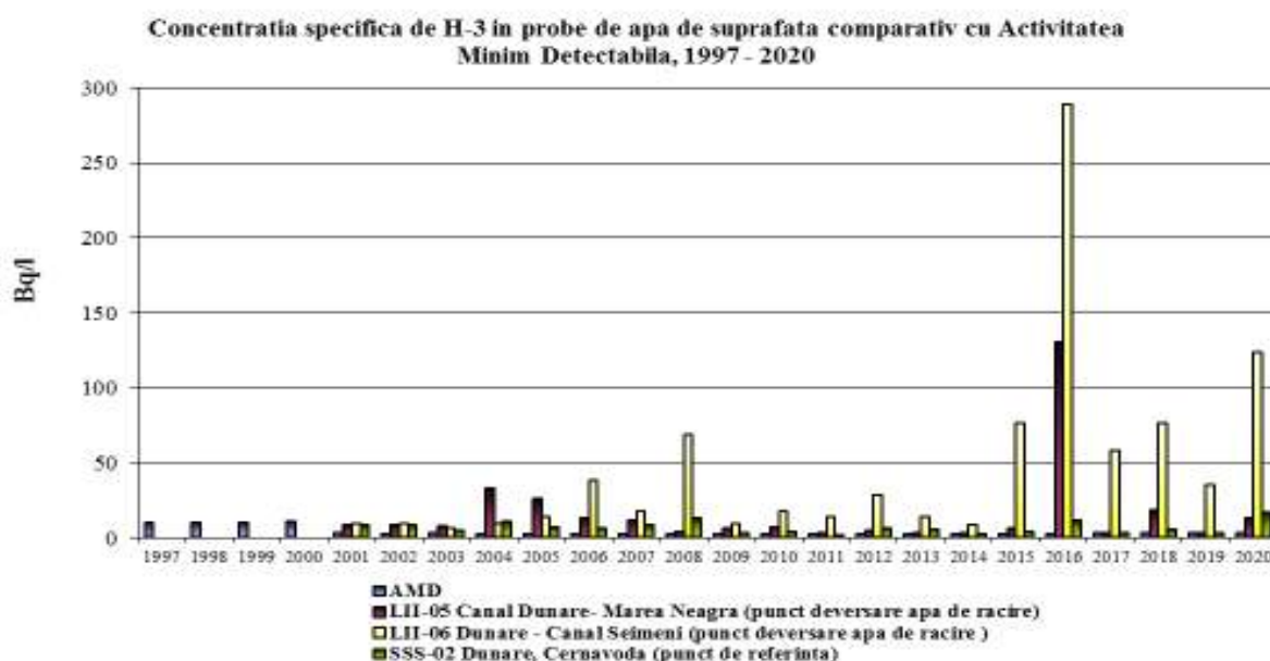
Figure 3.1.3.1.1 Annual average values of tritium concentration in surface water samples
