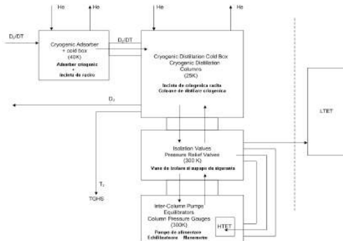
Figure 1.2.2.3.2 Schematic diagram of the cryogenic distillation system - CDS
