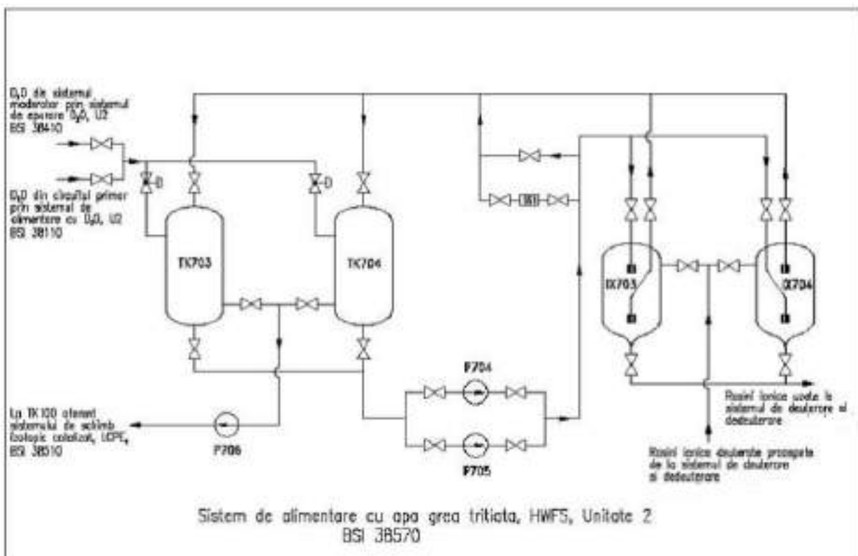
Figure 1.3.1.3 HWFS Tritiated Heavy Water Feed System (Unit 2)
