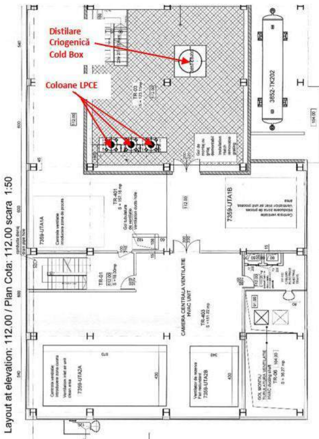
Figure 1.3.1.5 Catalytic isotopic exchange columns. Horizontal section through the CTRF building
