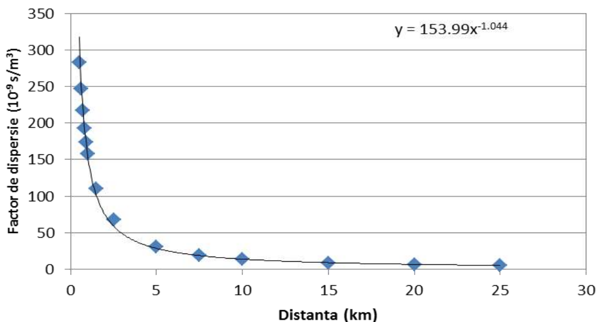
Figure 1.4.14.1 Simulation of atmospheric dispersion of tritium
