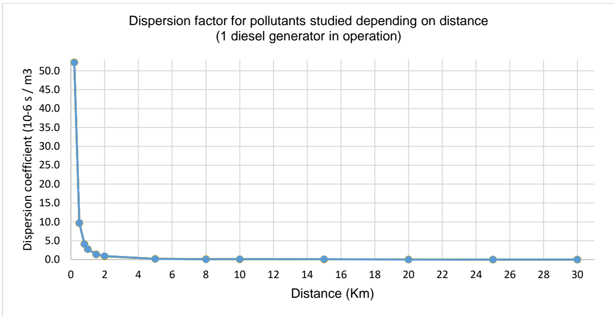
Figure 1.4.13.1 Distribution of the dispersion coefficient according to the distance from the stack at ground level (1 Diesel generator in operation)
