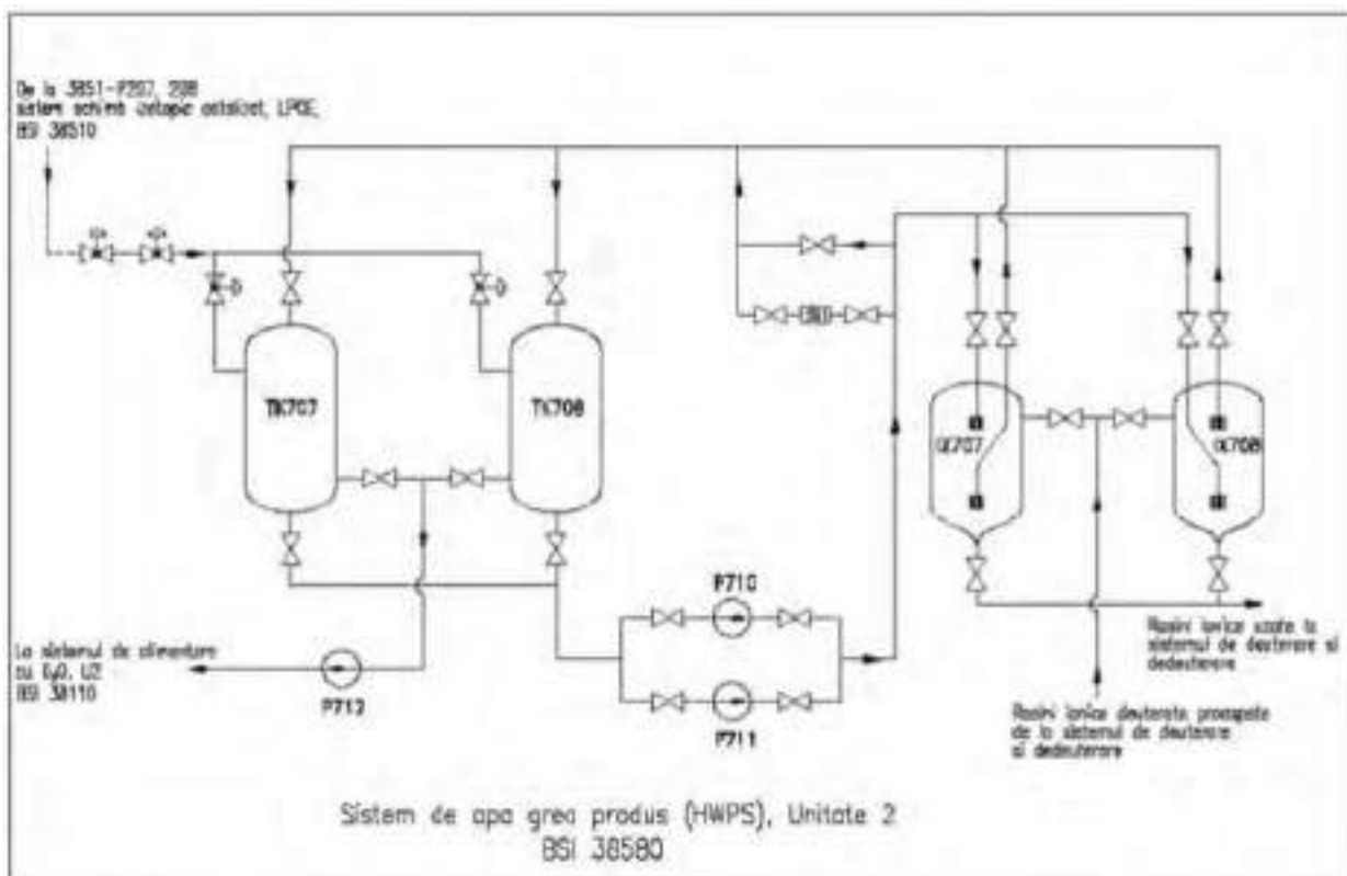
Figure 1.3.1.8 Product heavy water supply system (detritiated heavy water) HWPS - Unit 2
