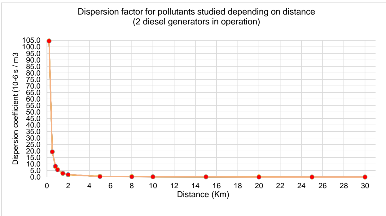
Figure 1.4.13.2 Distribution of the dispersion coefficient according to the distance from the stack at ground level (2 Diesel generators in operation)
