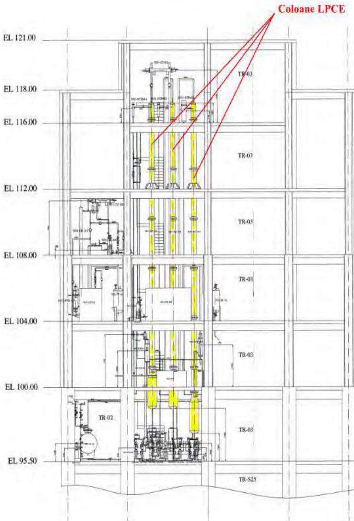
Figure 1.3.1.4 Catalytic isotopic exchange columns. Vertical section through the CTRF building
