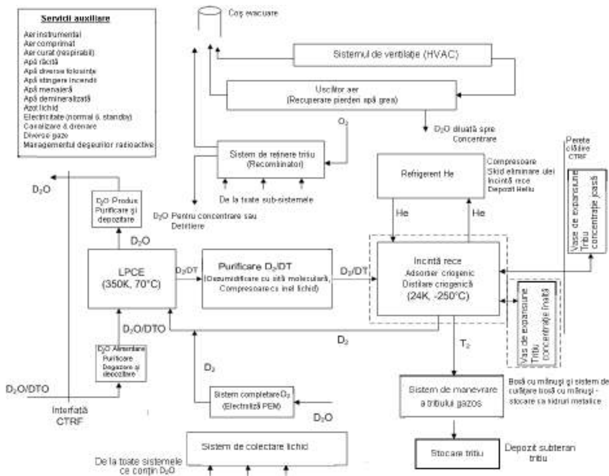
Figure 1.3.1.1 CTRF block diagram
