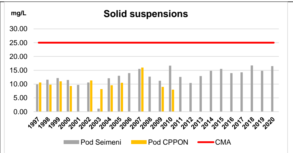
Figure 3.1.4.6. Annual average values for the concentration of solid suspensions in the liquid effluent
