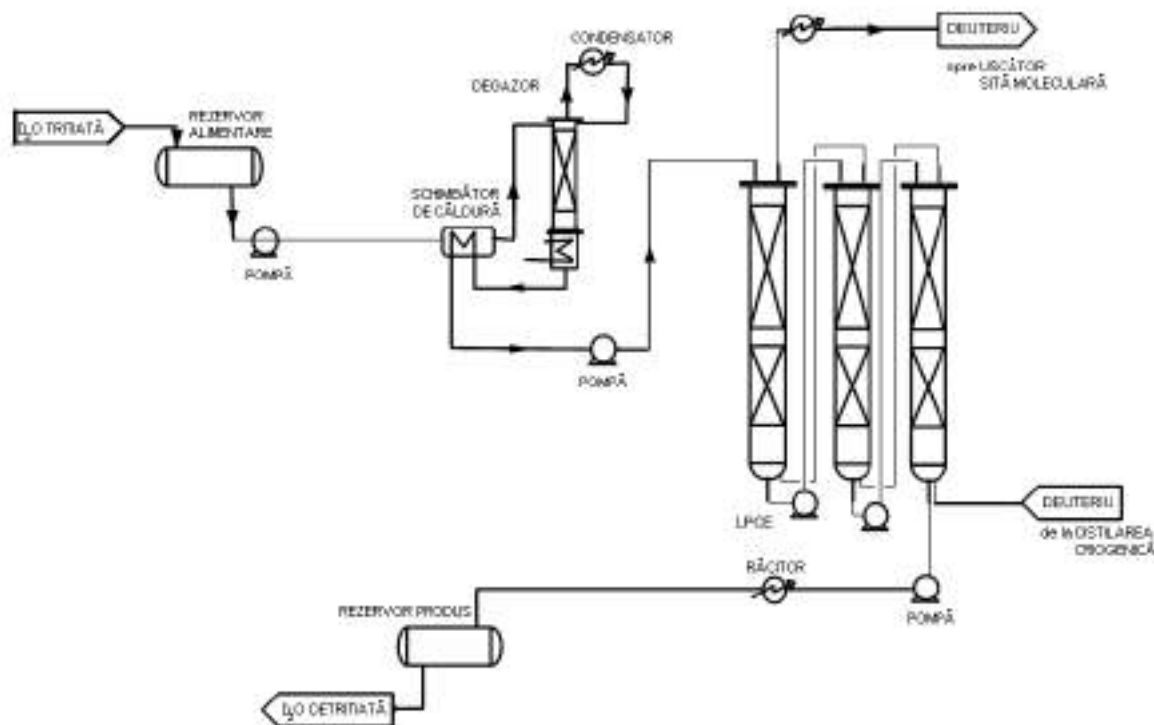
Figure 1.2.2.3.1 Schematic diagram of the isotope exchange system-LPCE
