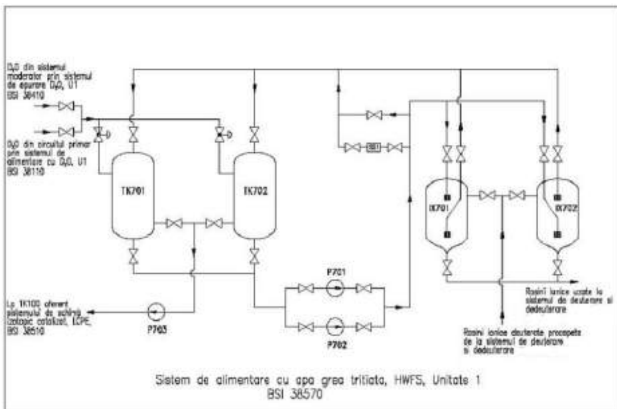
Figure 1.3.1.2 HWFS Tritiated Heavy Water Feed System (Unit 1)
