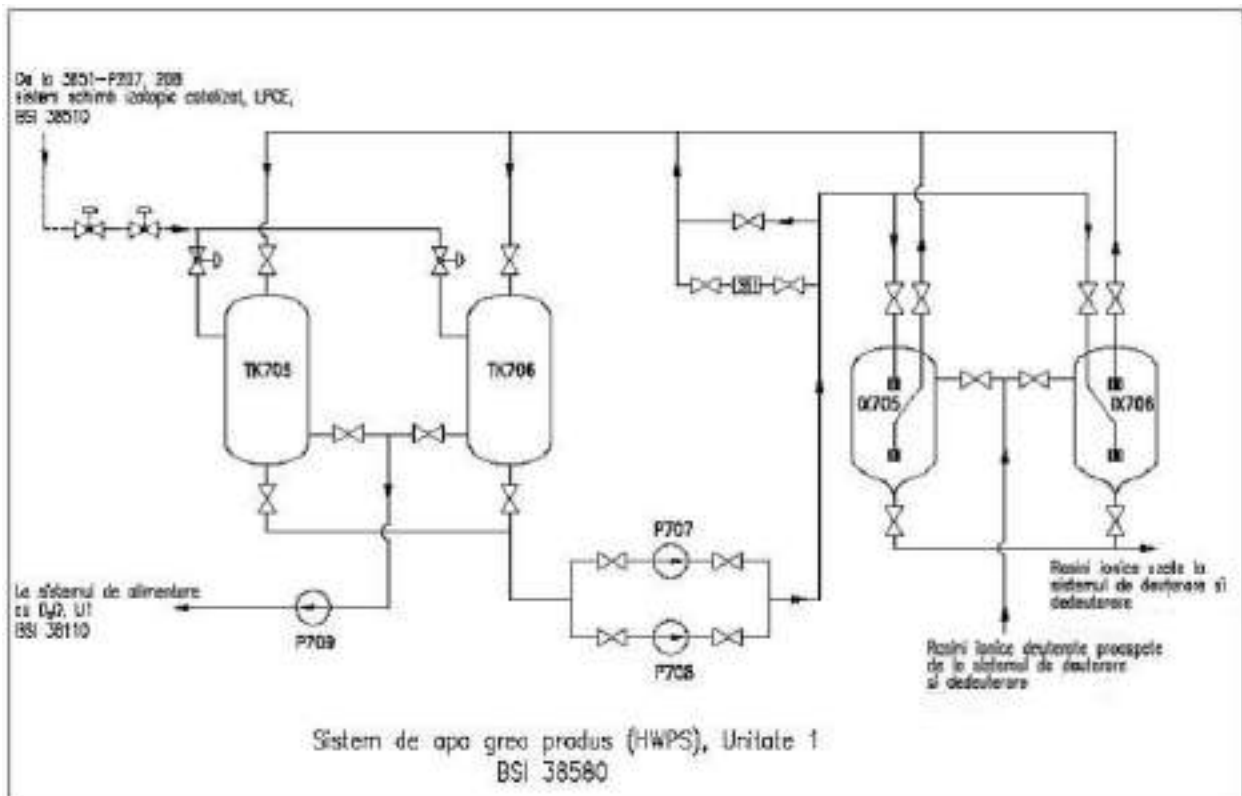
Figure 1.3.1.7 Product heavy water supply system (detritiated heavy water) HWPS - Unit 1
