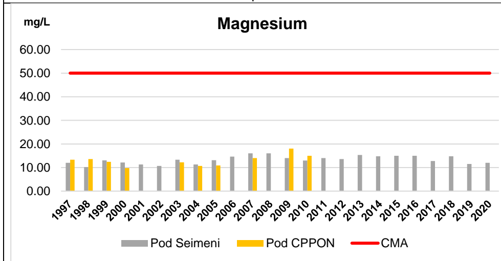
Figure 3.1.4.11. Annual average values for magnesium concentration in the liquid effluent
