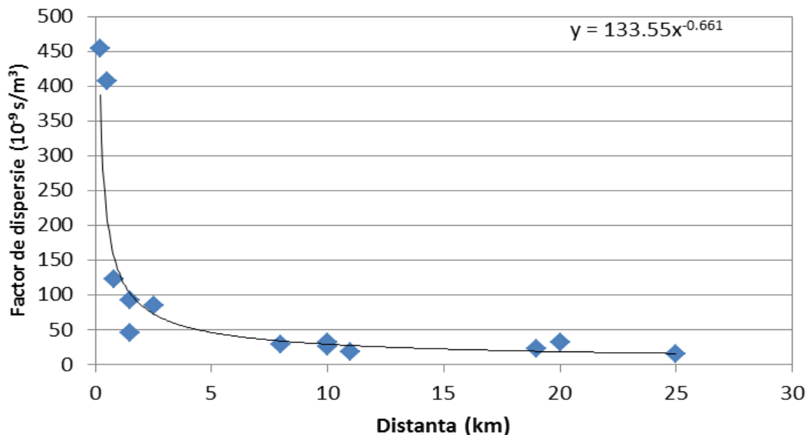
Figure 1.4.14.3 Distance variation of empirical atmospheric dispersion factors, determined based on the monitoring data from 2006-2018
