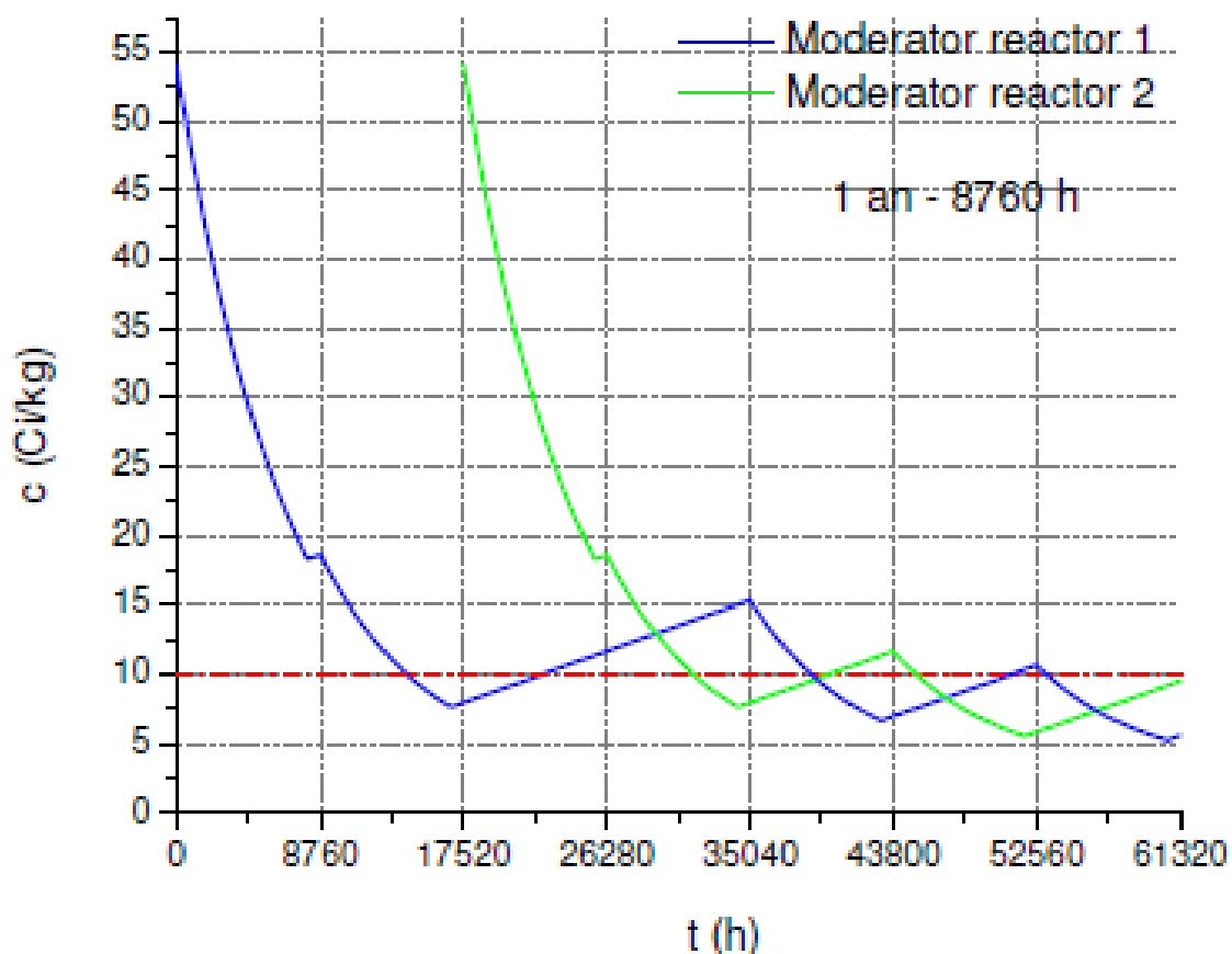
Figure 4.8.1 CTRF operating chart for reactors 1 and 2 with proposed operating target of 10 Ci/kg [2].
