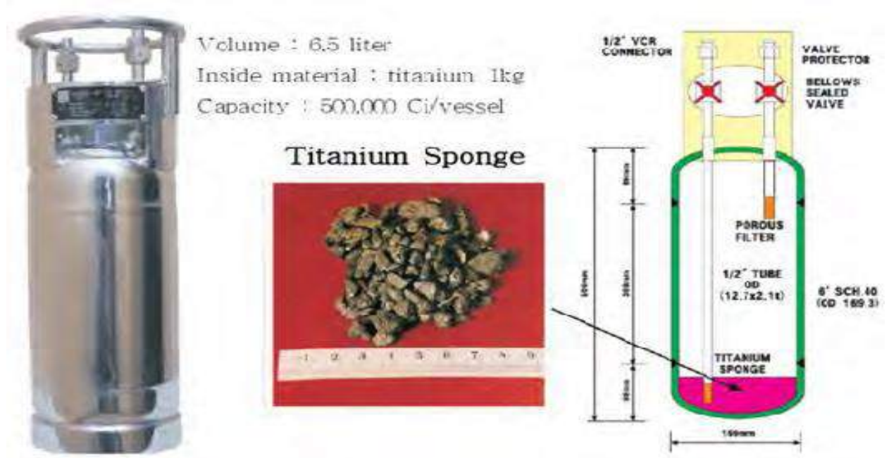
Figure 1.3.1.6 Container model for storing tritium on a titanium bed at WTRF-Korea
