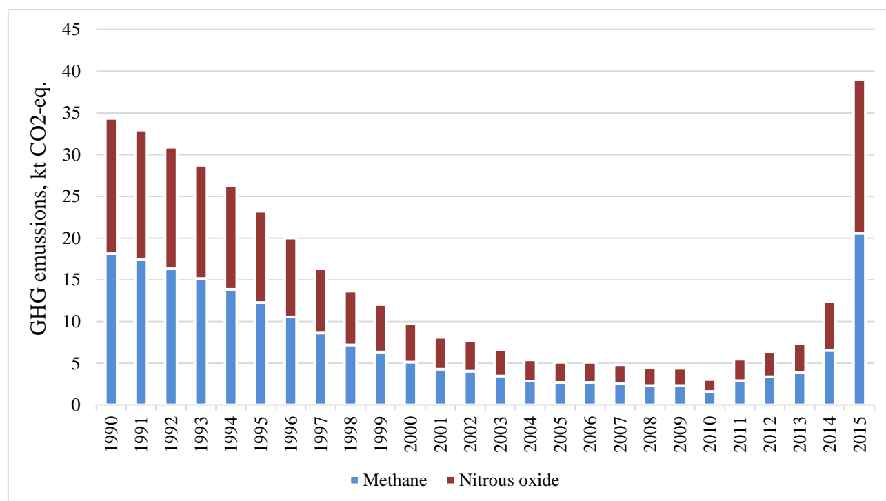
Fig. 7.8. GHG emissions from waste composting in Ukraine, 1990-2015.
